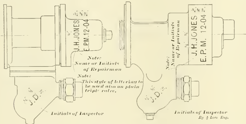
WESTINGHOUSE TRIPLE VALVE.
